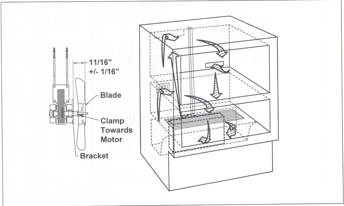
Figure 5-1. 700BR-2 Air Flow and Fan Blade Spacing
