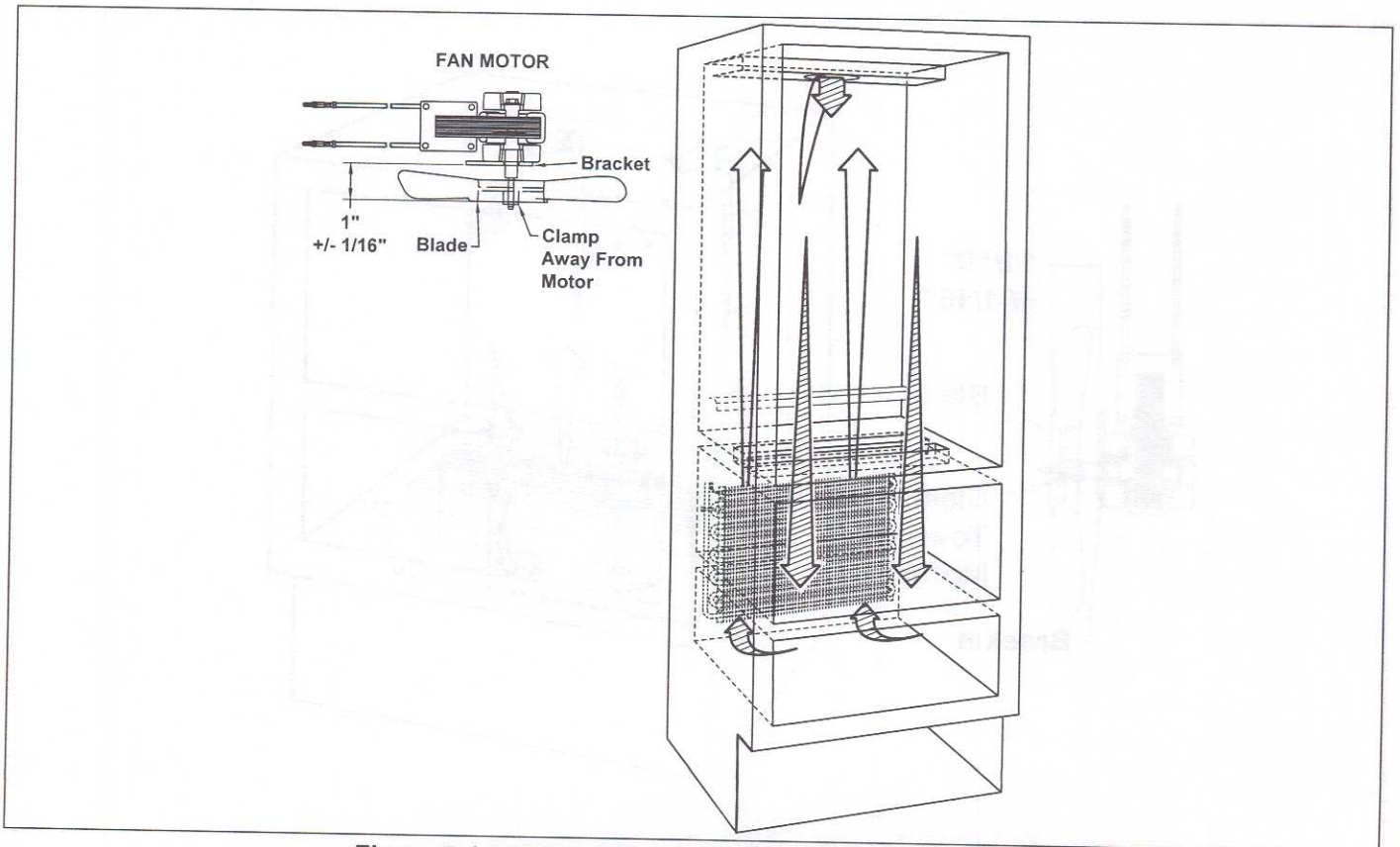
Figure 5-1. 700TF/I-2 Air Flow and Fan Blade Spacing
