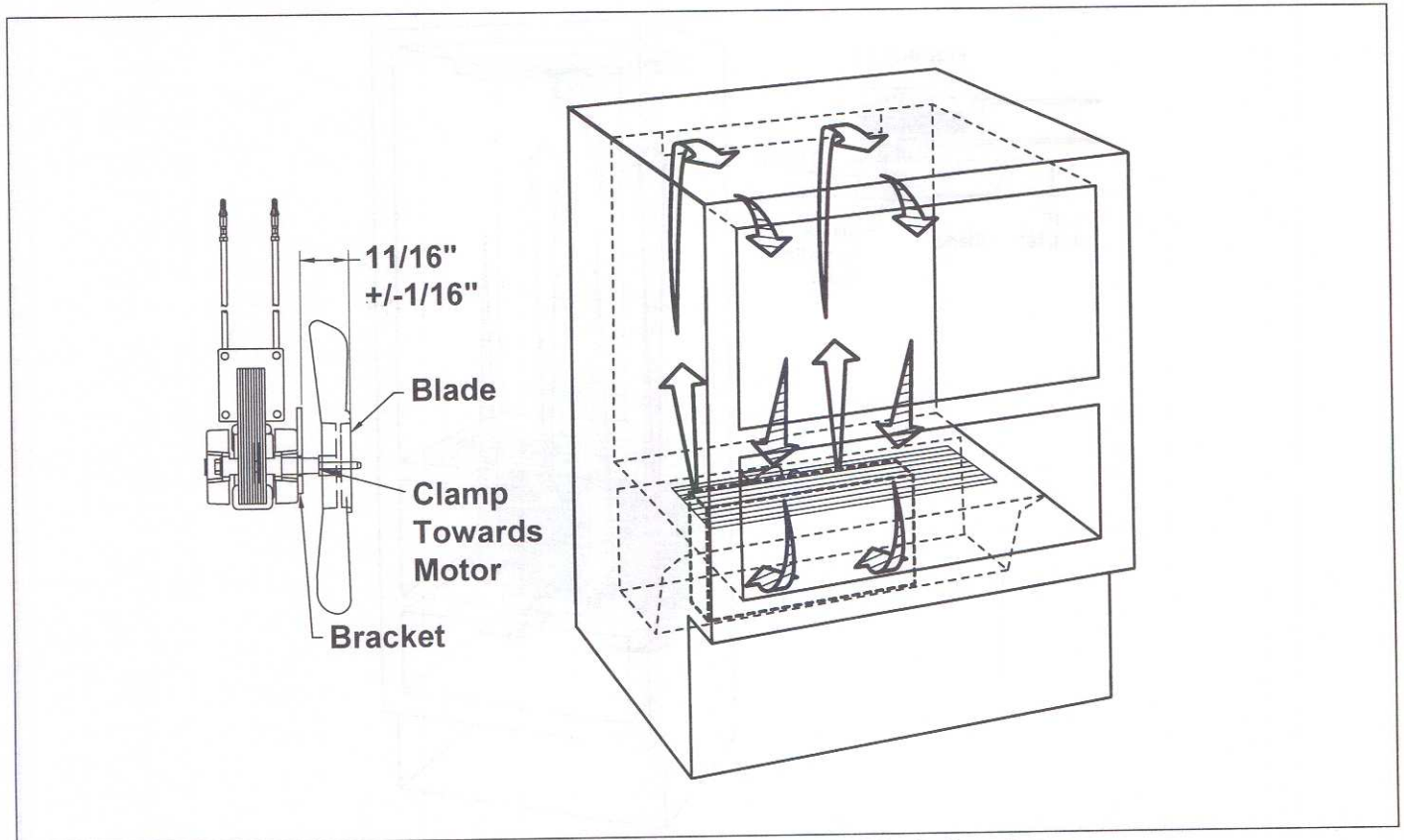
Figure 5-1. 700BF/I-2 Air Flow and Fan Blade Spacing
