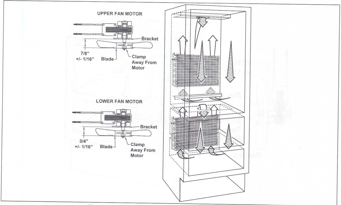
Figure 5-1. 700TR-2 Air Flow and Fan Blade Spacing
