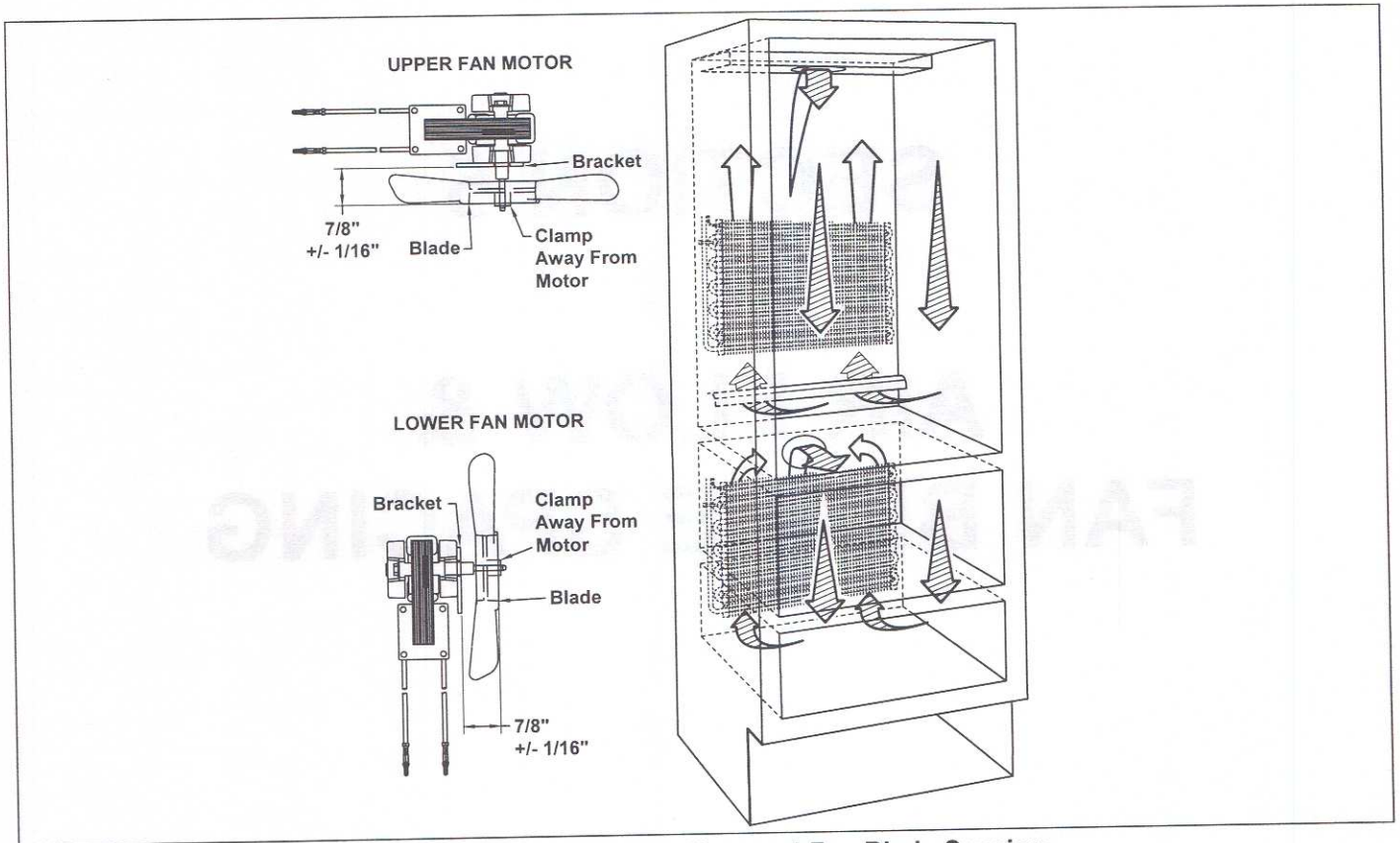
Figure 5-1. 700TC/I-2 Air Flow and Fan Blade Spacing
