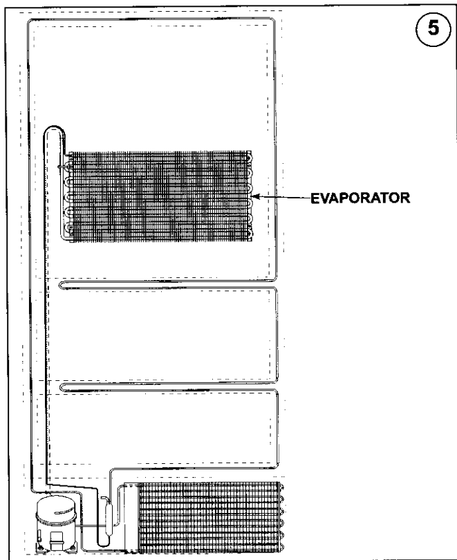
Figure 4-5. Evaporator
