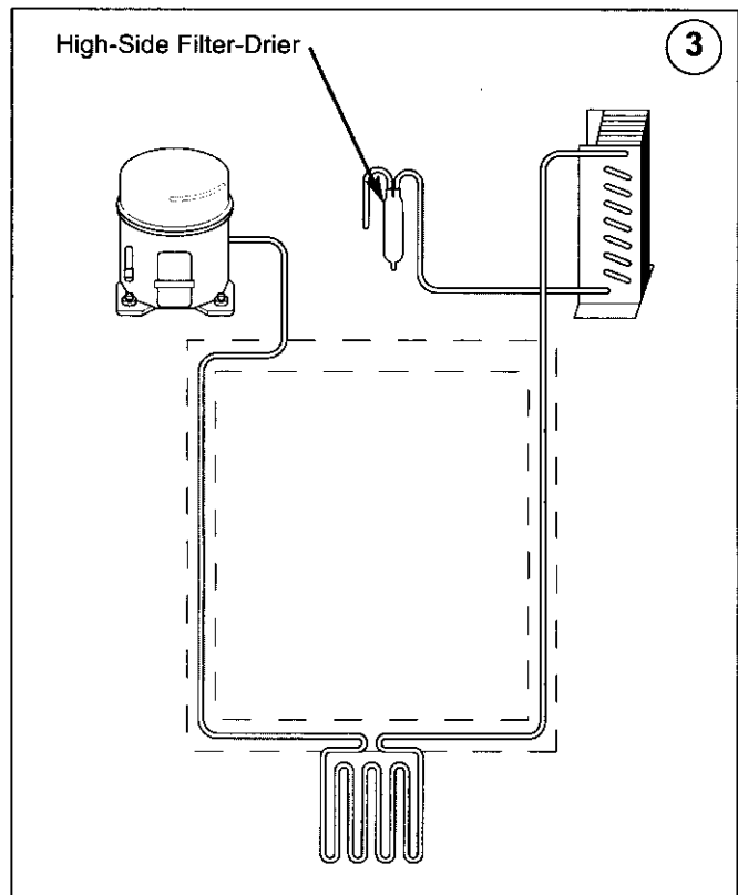
Figure 4-3. High-Side Filter-Drier
